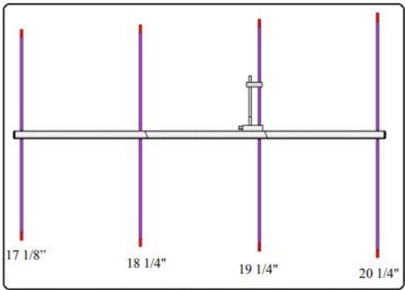
4 Element Portable Antenna for 2 meters
