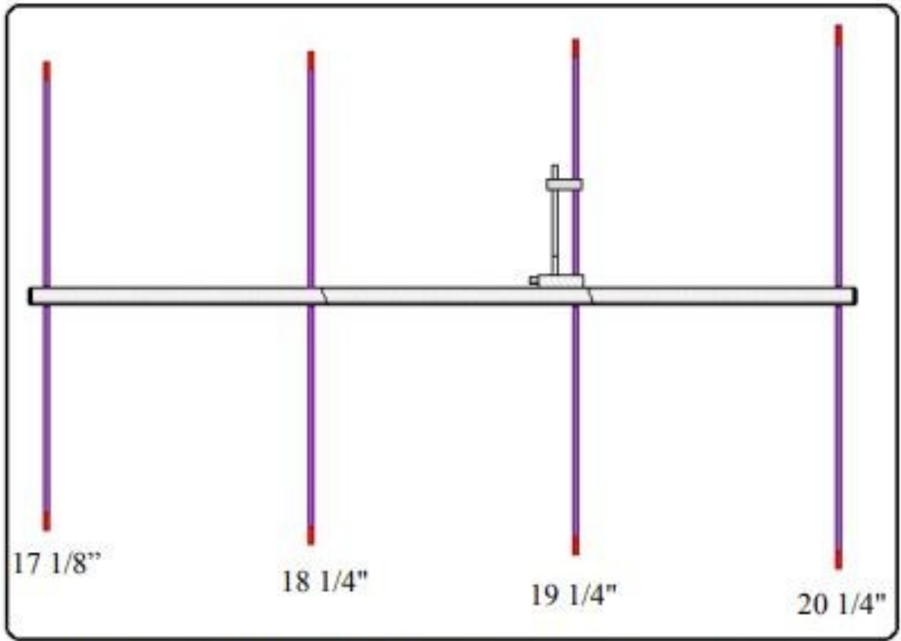
4 Element Portable Antenna for 2 meters
